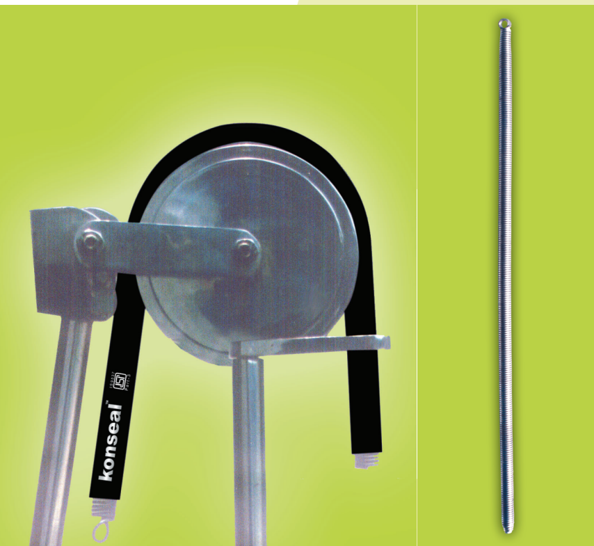
Conduit bending with the aid of spring and test apparatus.
